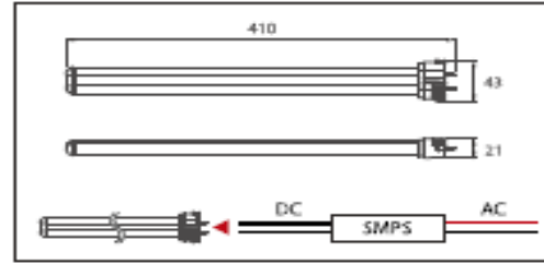
410mm
